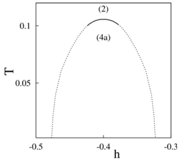
Fig. 7. Phase diagram in the (T-h) plane at \Omega = 0 . The parameter values are: g = -0.4 , W = 1 , \mu = 0 . The notations are the same as in Figs. 1 and 2
