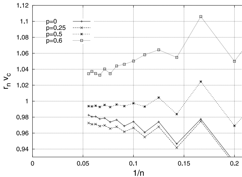
Figure 5. Ratio approximants for different dilutions p vs. 1/n (normalized by v_c as in figure 3).
