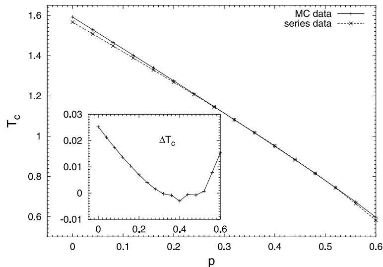
Figure 6. Transition temperatures of the bond-diluted 4-state Potts model for different dilution p as obtained from Monte Carlo (MC) simulations [39] and DLog-Padé series analysis. The inset shows the difference between the two estimates.
