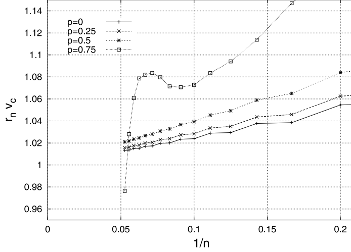
Figure 3. Ratio approximants for different dilutions p vs. 1/n . In order to make them visually comparable, they are (except for p = 0.75 ) normalized by their respective critical couplings v_c .
