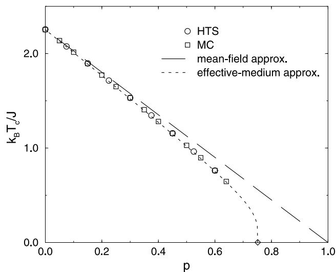
Figure 4. Transition temperatures of the bond-diluted Ising model for different dilutions p as obtained from our DLog-Padé high-temperature series (HTS) analysis and from Monte Carlo (MC) simulations [26]. For comparison the (properly normalized) mean-field and effective-medium approximations are shown as well.
