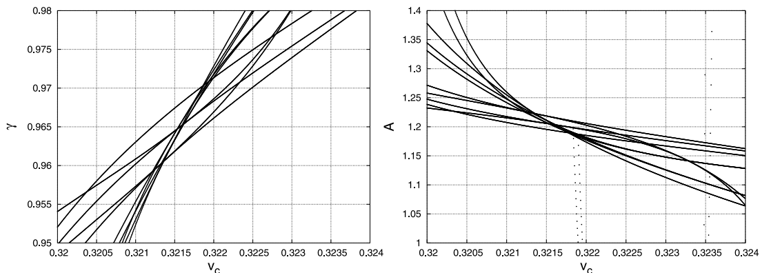
Figure 8. Values for the critical exponent \gamma and amplitude A at p = 0.4 as function of trial v_c estimates from the Baker-Hunter analysis. From the clustering of different Padé approximants in both pictures we estimate v_c = 0.3217 , \gamma = 0.966 , and A = 1.21 .
