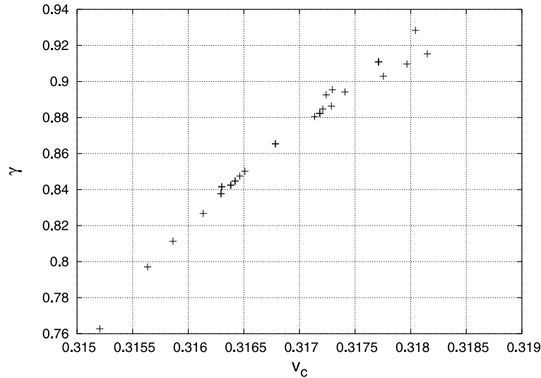
Figure 7. Scattering of different Padé approximants at dilution p = 0.4 : critical exponent \gamma against critical coupling v_c .
