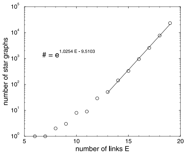
Figure 1. Growth behaviour of the number of star graphs with E links that can be embedded in hypercubic lattices \mathbb{Z}^d .
