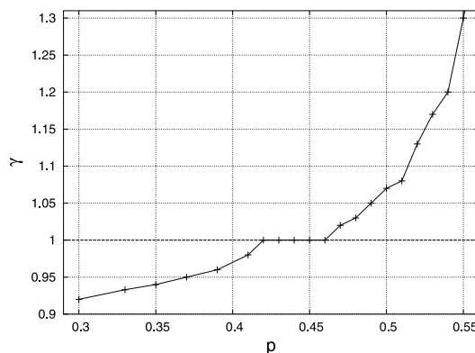
Figure 9. Effective critical exponent \gamma as function of the dilution p from Baker-Hunter analysis.
