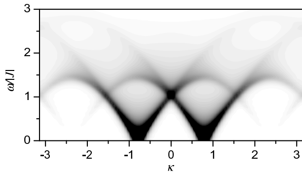
Figure 2. S_{xx}(\kappa, \omega) for \Omega = 0.001 , J = -1 , D = 1 , \beta = 20 .
