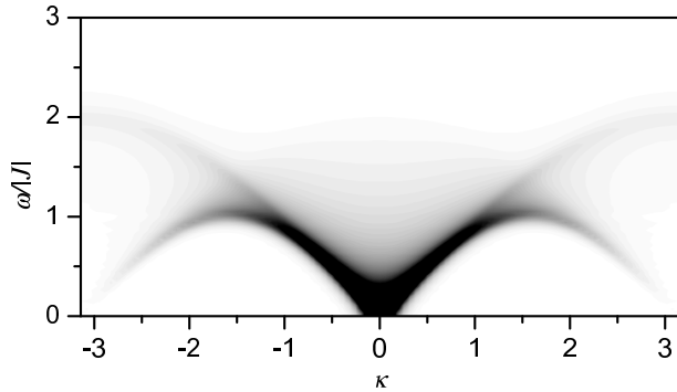
Figure 1. S_{xx}(\kappa, \omega) for \Omega = 0.001 , J = -1 , D = 0 , \beta = 20 .
