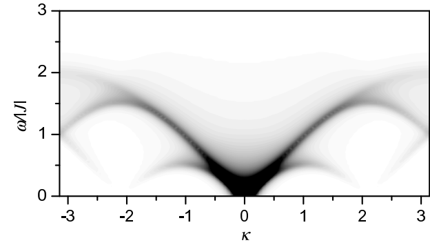
Figure 3. S_{xx}(\kappa, \omega) for \Omega = 0.5 , J = -1 , D = 0 , \beta = 20 .
