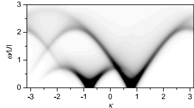
Figure 4. S_{xx}(\kappa, \omega) for \Omega = 0.5 , J = -1 , D = 1 , \beta = 20 .
