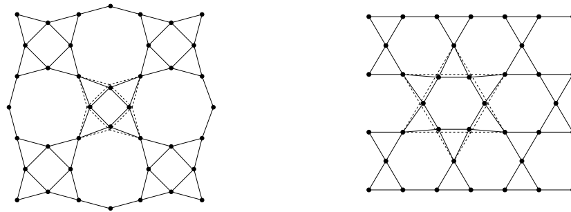
Figure 1. Square-kagomé lattice with one distorted square (left) and kagomé lattice with one distorted hexagon (right) which can host localized magnons. The parts of the lattices before distortions are shown by dashed lines. All bonds in the lattices before distortions have the same length.
